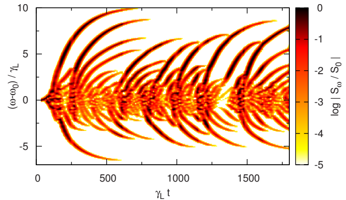
FIG. 12. (Color online) Logarithmic scale plot of the time evolution of the frequency power spectrum for \gamma_d=0.938\gamma_L^* , \nu_a=2.7 \times 10^{-3}\gamma_L^* . At each time, the spectrum is normalized to its maximum value.
